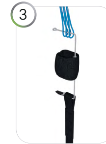
3 Push now the IKS line through the lines and the riser. The reinforced end with the black tab should be located on the riser side.
