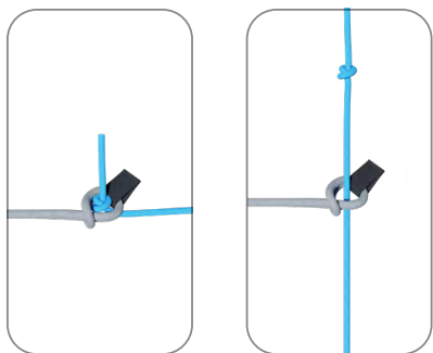
Diagram 1. Speed-bar connection by means of Kite loop (without Brummel hook)
