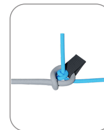
Diagram 2. Speed-bar connection by means of kite loop (without Brummel hook).
