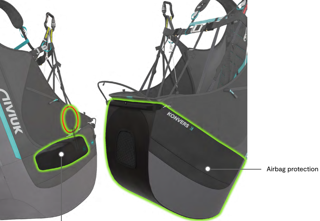
Rescue compartment
