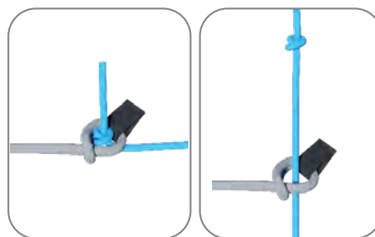
1. A knot is tied in the speed-bar cord and passed through the connector of the webbing cord. 2. Tension is applied to both sides of the system until the knot tightens against the riser connector.
